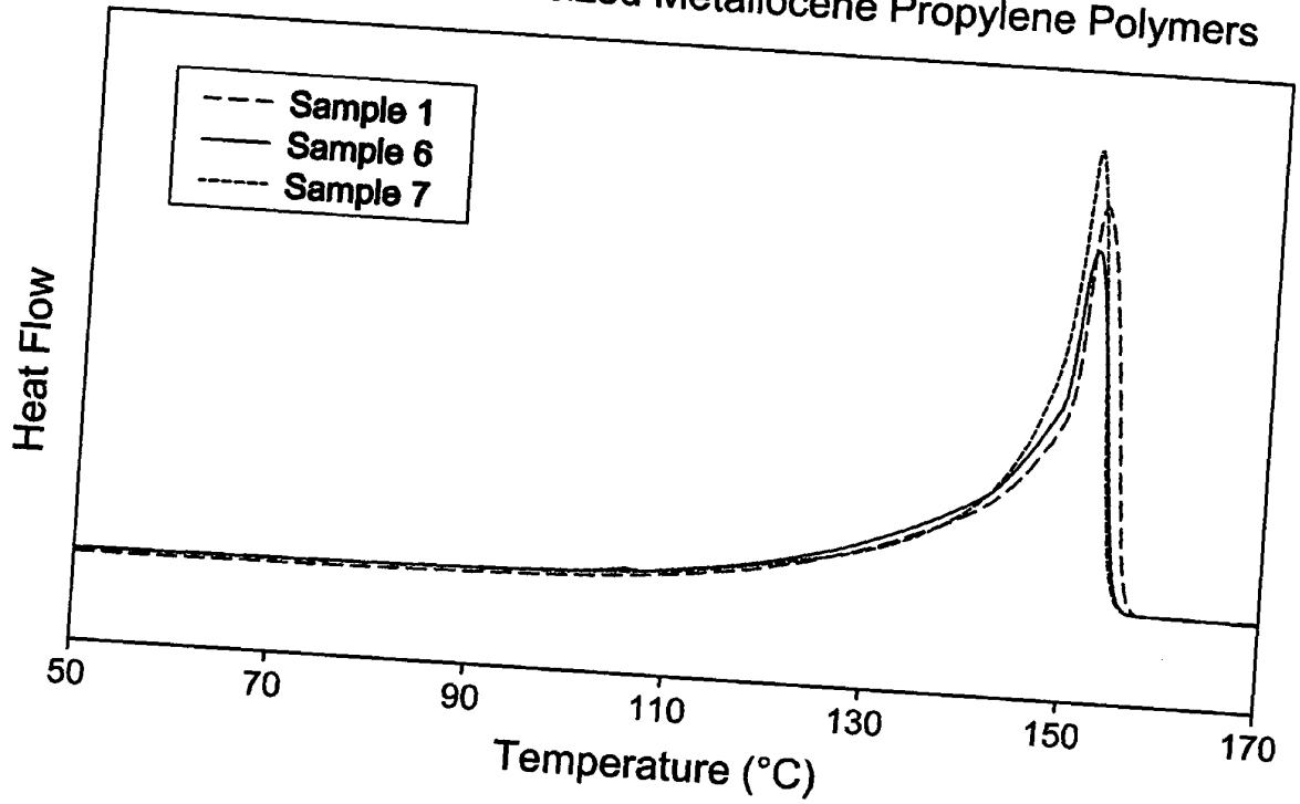
Fig. 6 DSC Crystallization of Plasticized Metallocene Propylene Polymers
